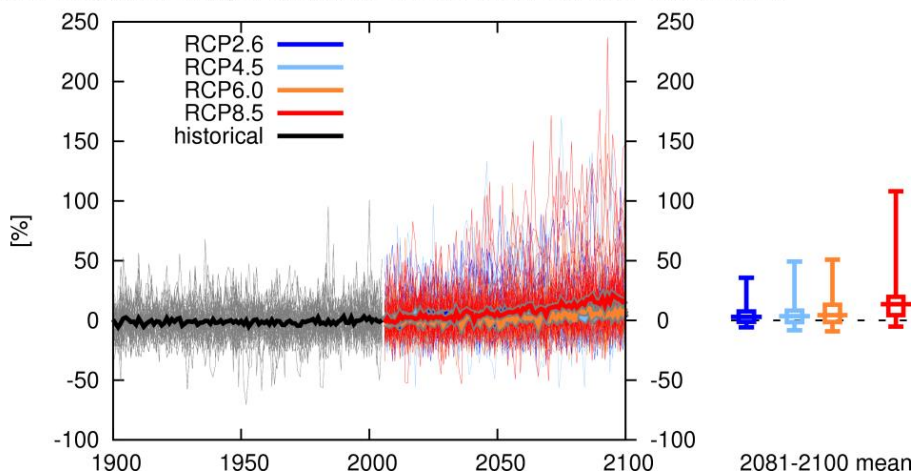
Relative Precipitation change Ethiopia Jan-Dec wrt 1986-2005 AR5 CMIP5 subset
